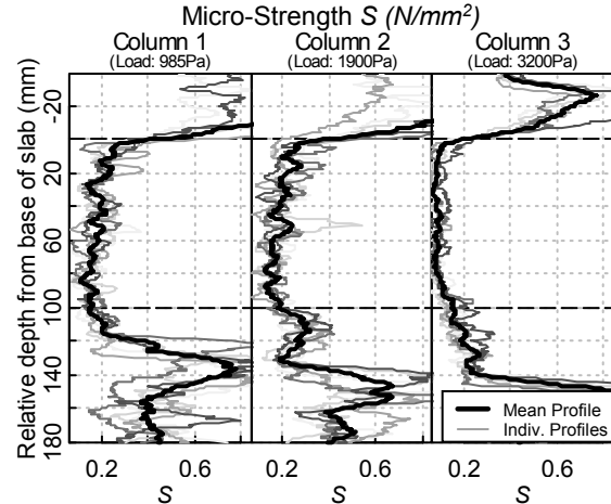
Figure 6. Micro-scale strength S . Horizontal lines approximate depth hoar boundaries.
