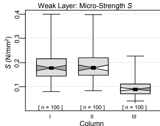
Figure 7. Micro-scale strength S ( N/mm^2 ) of weak layer. The loaded column (III) possessed the lowest S values while the unloaded and natural columns (I and II) were indistinguishable.
