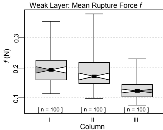
Figure 3. Mean rupture force f of weak layer. The unloaded column (I) possessed the highest average f values while the loaded column (III) maintained the smallest values
