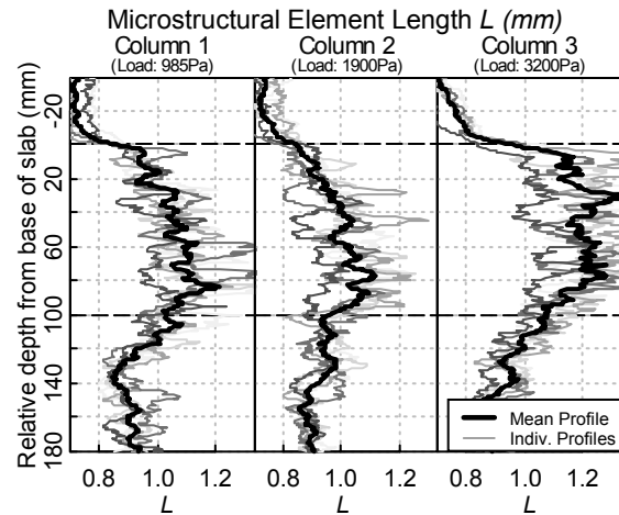
Figure 4. Microstructural element length L . Horizontal lines approximate depth hoar boundaries.
