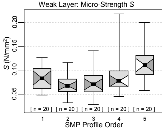
Figure 8. Weak layer micro-strength of Column III, grouped by sample (SMP profile) order (approximately 8 minutes between profiles).
